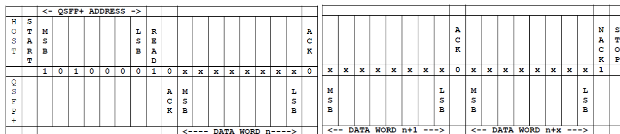
Figure 4: Sequential Address Read Starting at QSFP+ Current Address
